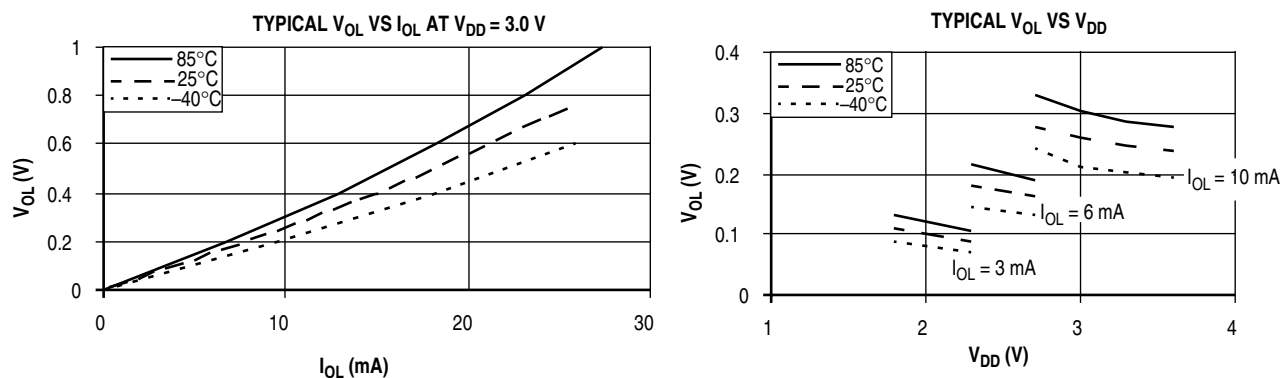
Figure A-2. Typical Low-Side Driver (Sink) Characteristics (Port C)
