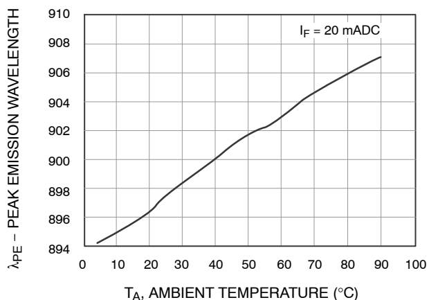
Figure 2. Peak Wavelength vs. Ambient Temperature
