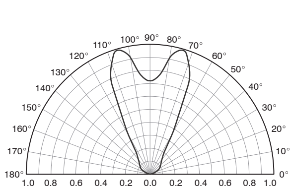
Figure 7. Radiation Diagram
