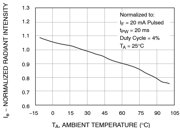
Figure 4. Normalized Radiant Intensity vs. Ambient Temperature
