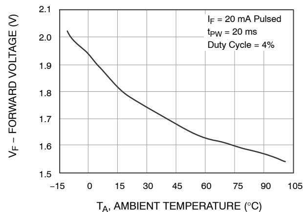
Figure 6. Forward Voltage vs. Ambient Temperature
