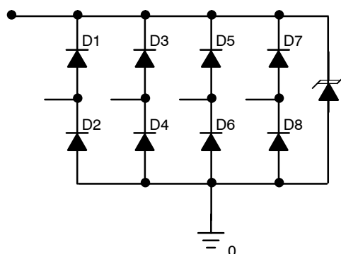
NUP4114UPXV6 Equivalent Circuit
