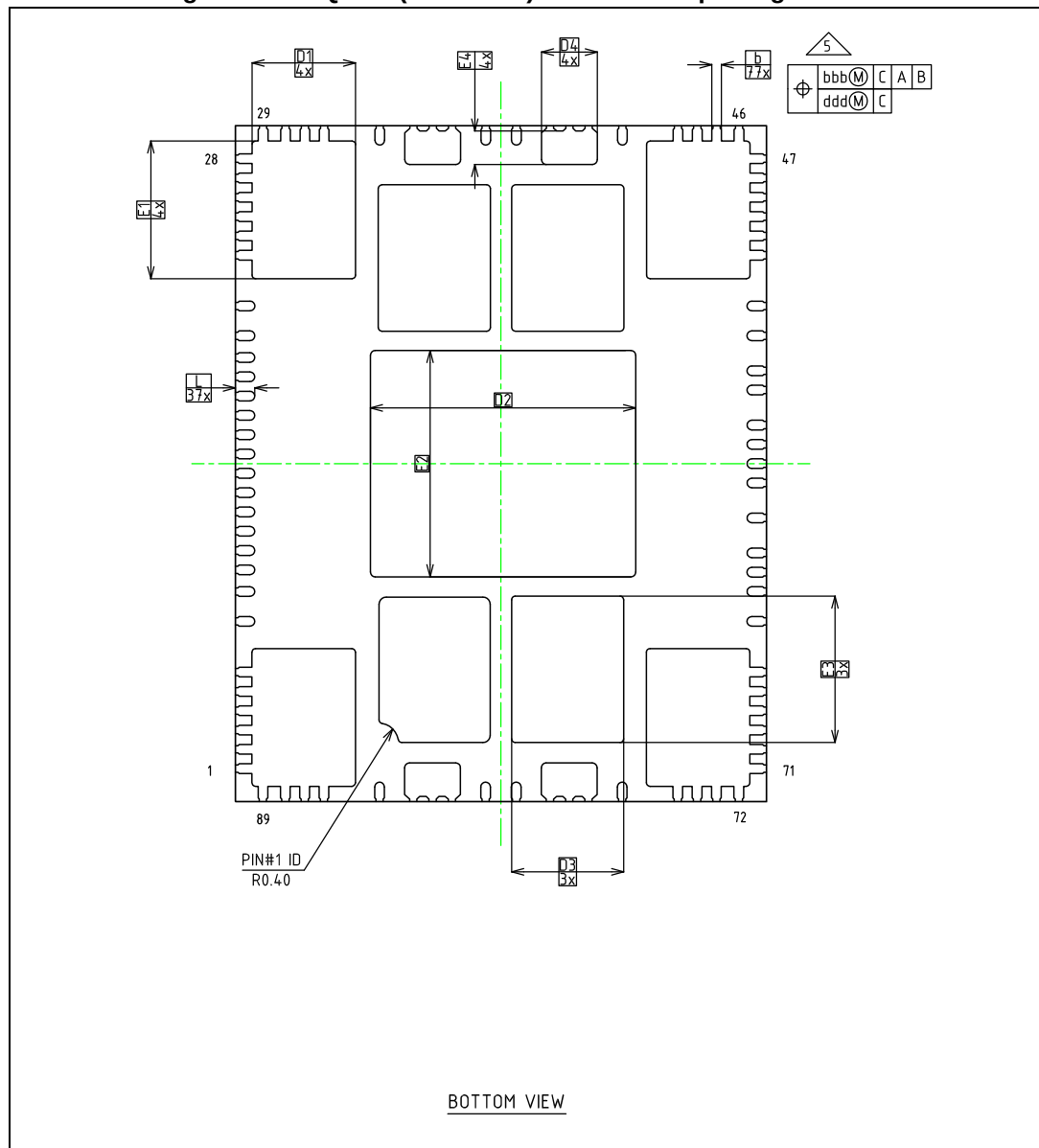
Figure 31. VFQFPN (11x14x1.0) bottom view package outline
