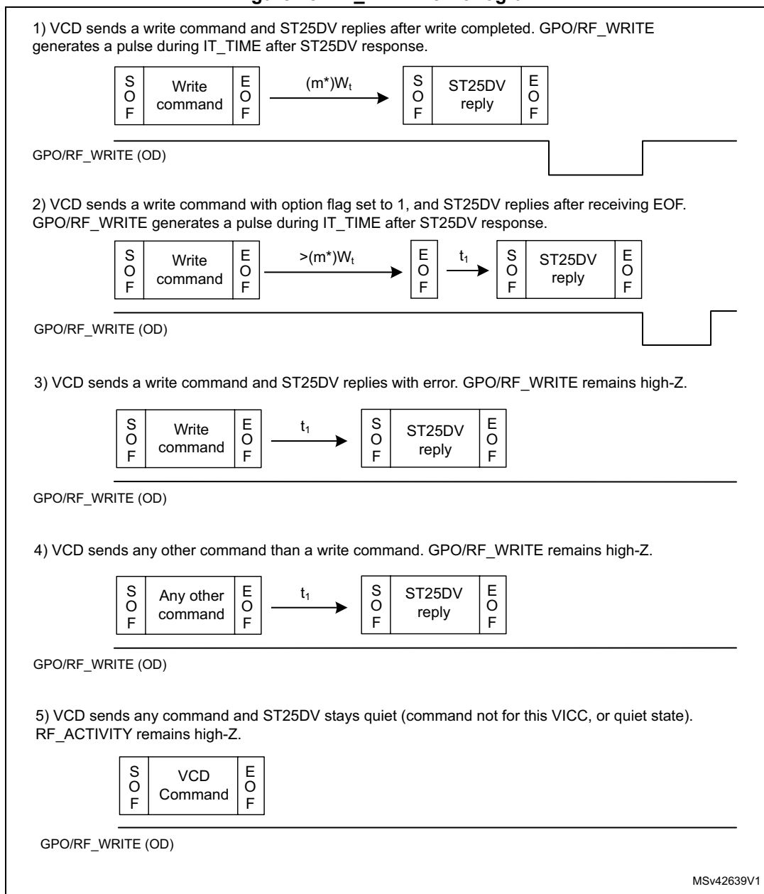
Figure 18. RF_WRITE chronogram
