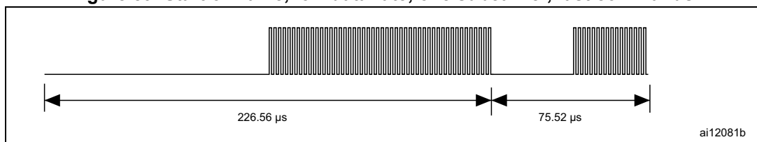
Figure 89. Start of frame, low data rate, one subcarrier, fast commands
