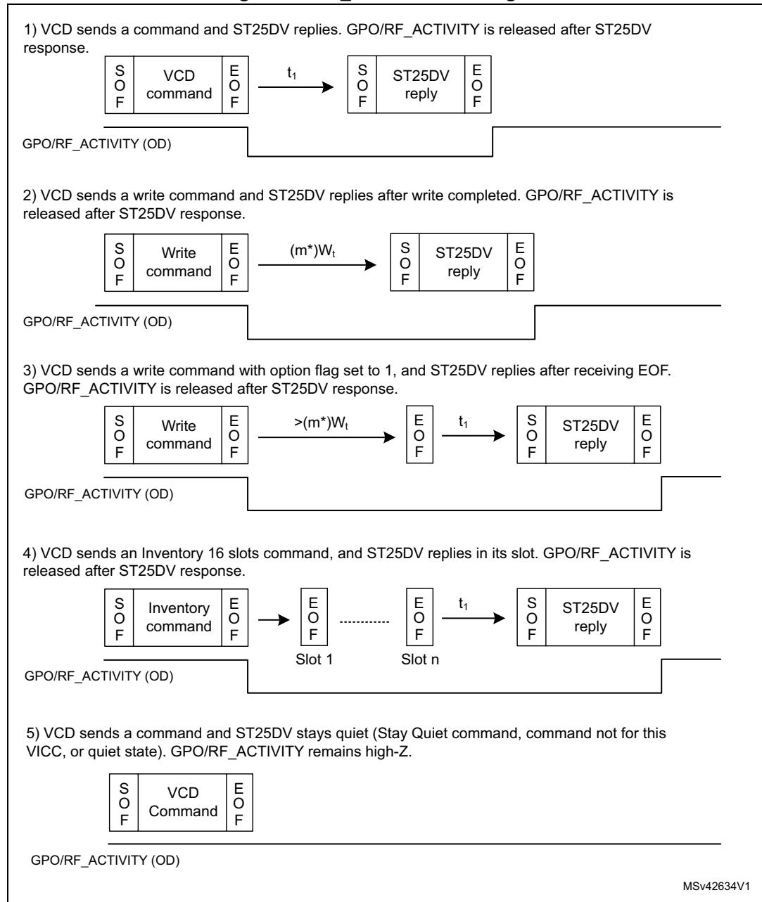
Figure 13. RF_ACTIVITY chronogram
