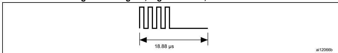
Figure 84. Logic 0, high data rate, fast commands
