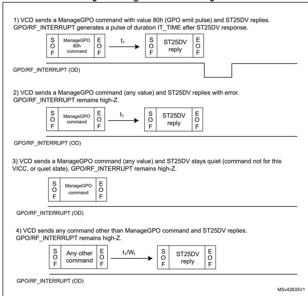
Figure 14. RF_INTERRUPT chronogram
