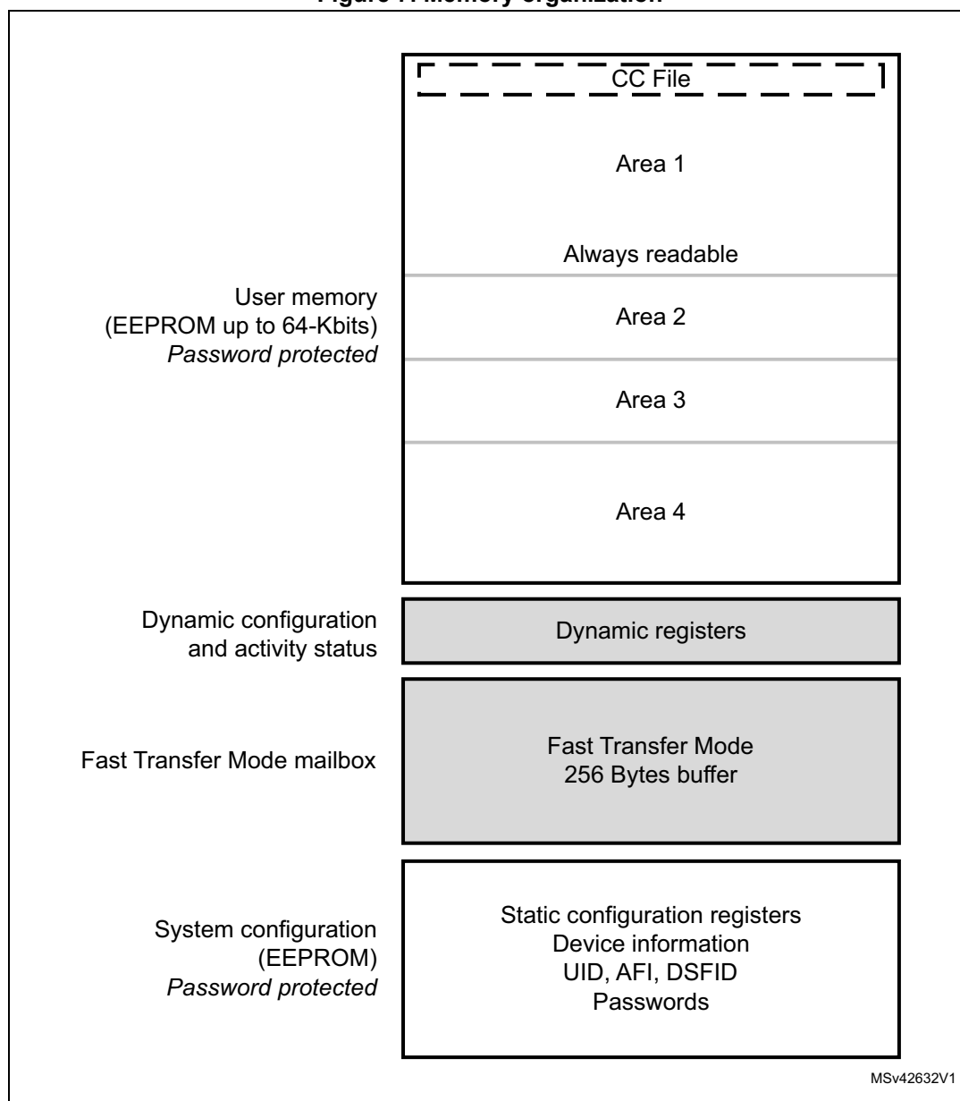
Figure 7. Memory organization
