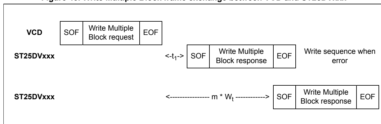
Figure 43. Write Multiple Block frame exchange between VCD and ST25DVxxx
