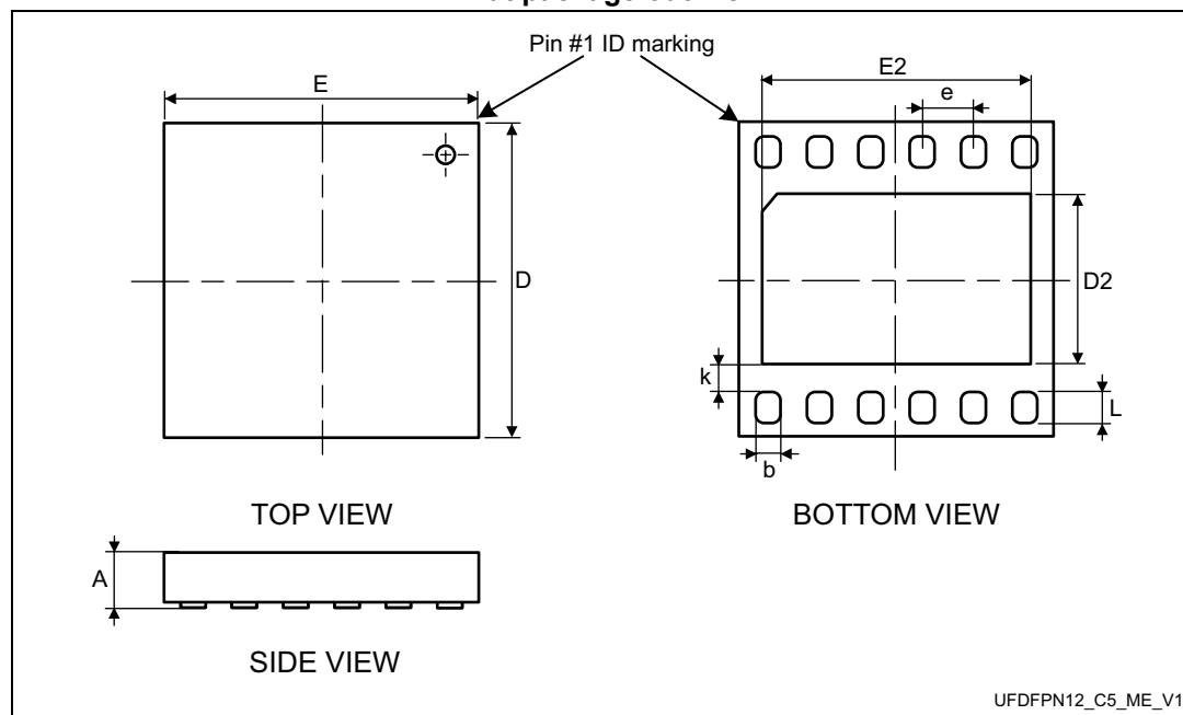
Figure 81. UFDFPN12 - 12-lead, 3x3 mm, 0.5 mm pitch ultra thin profile fine pitch dual flat package outline
