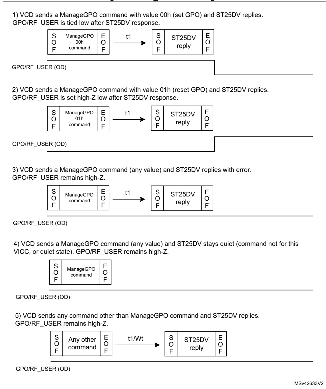
Figure 12. RF_USER chronogram
