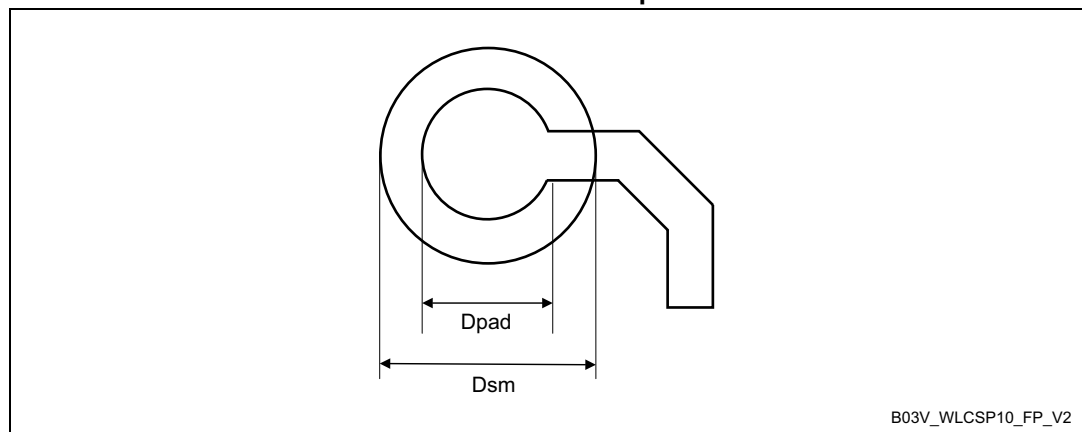
Figure 83. WLCSP - 10 balls, 1.649x1.483 mm, 0.4 mm pitch, wafer level chip scale recommended footprint
