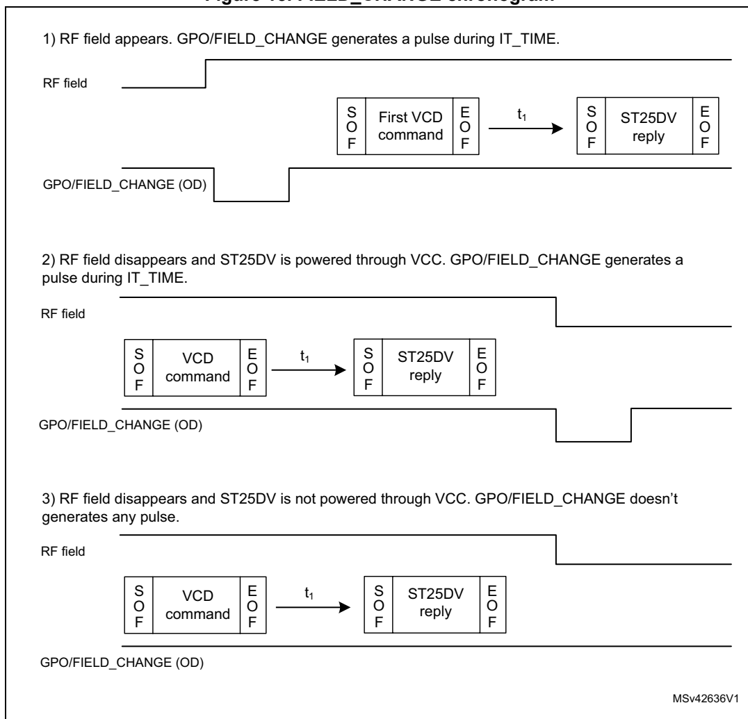
Figure 15. FIELD_CHANGE chronogram
