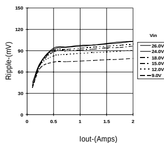
Ripple vs Output Current
