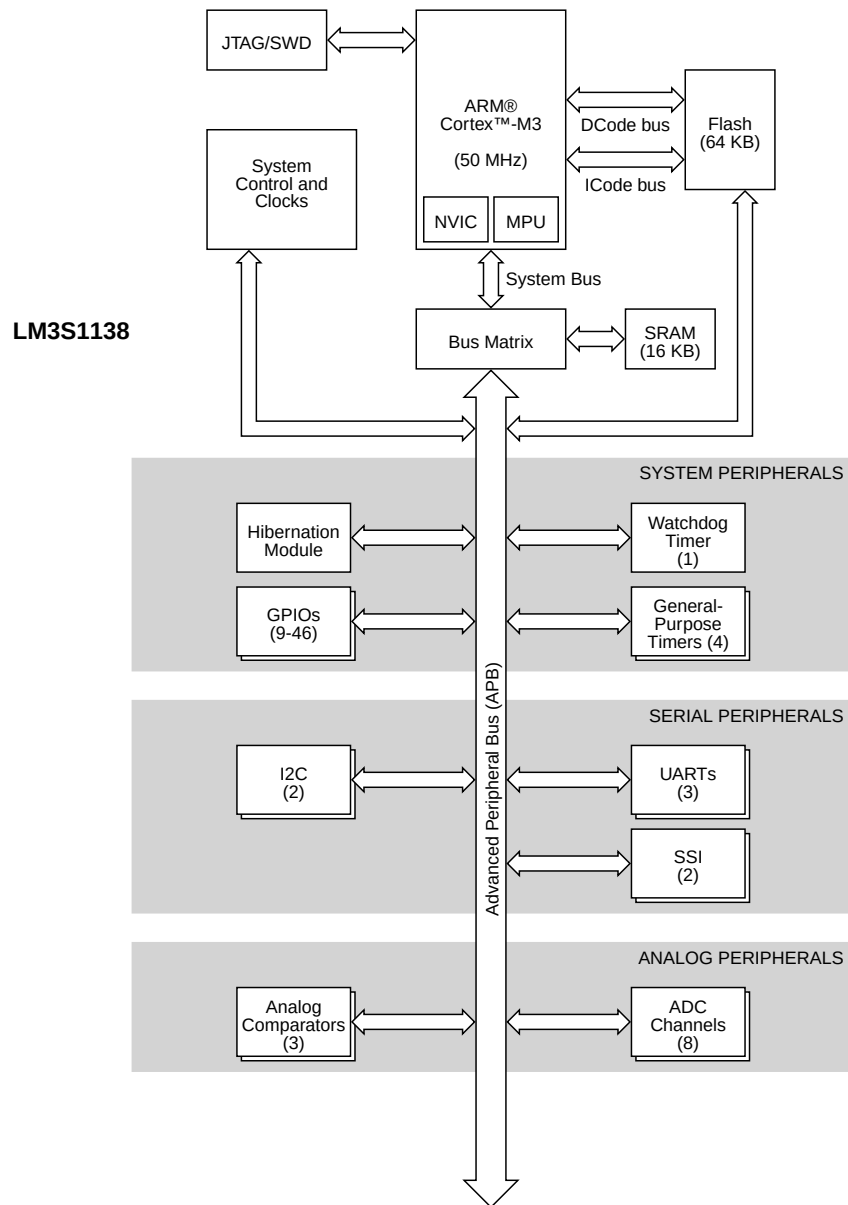
Figure 1-1. Stellaris® LM3S1138 Microcontroller High-Level Block Diagram
