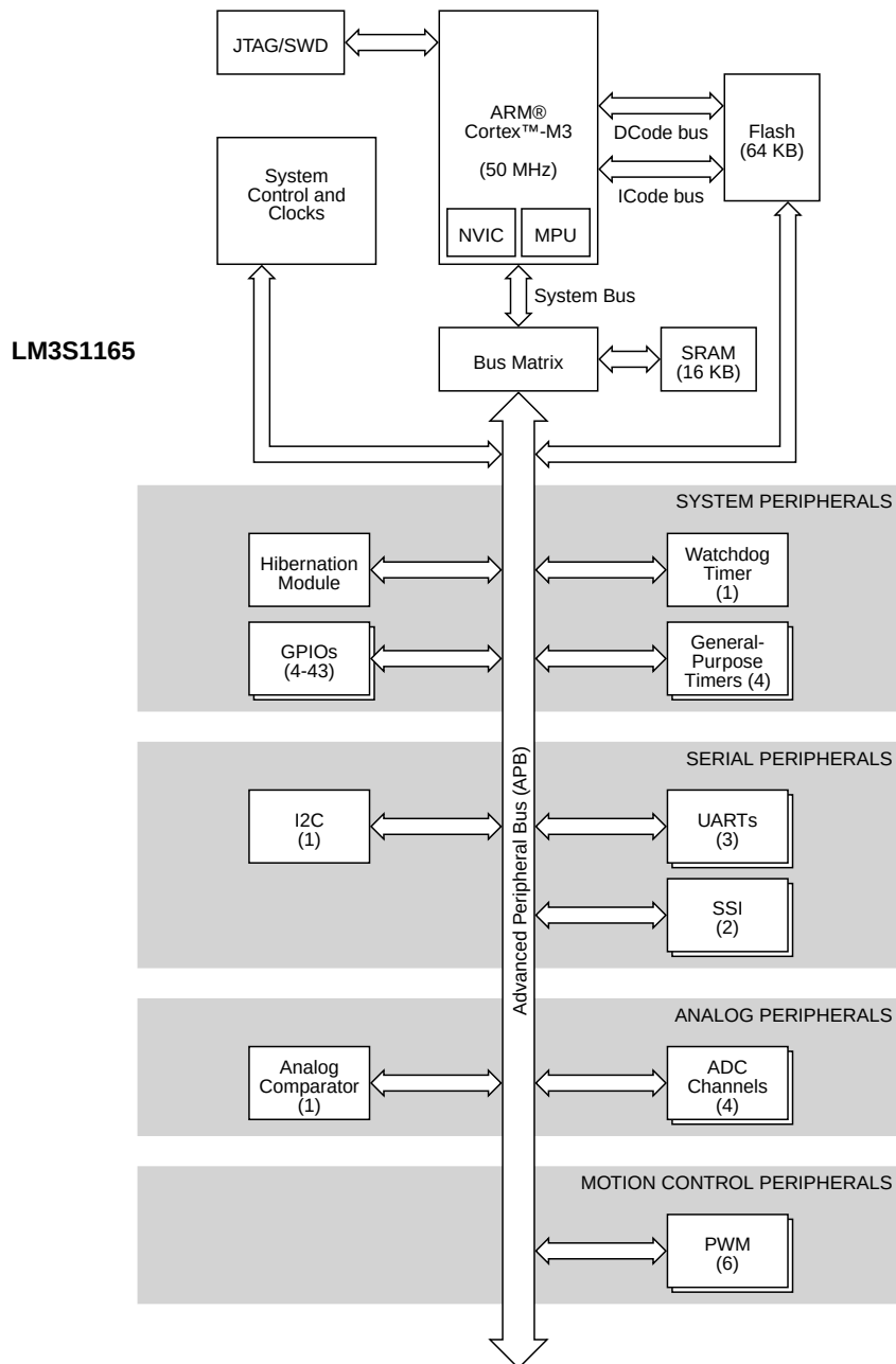
Figure 1-1. Stellaris® LM3S1165 Microcontroller High-Level Block Diagram
