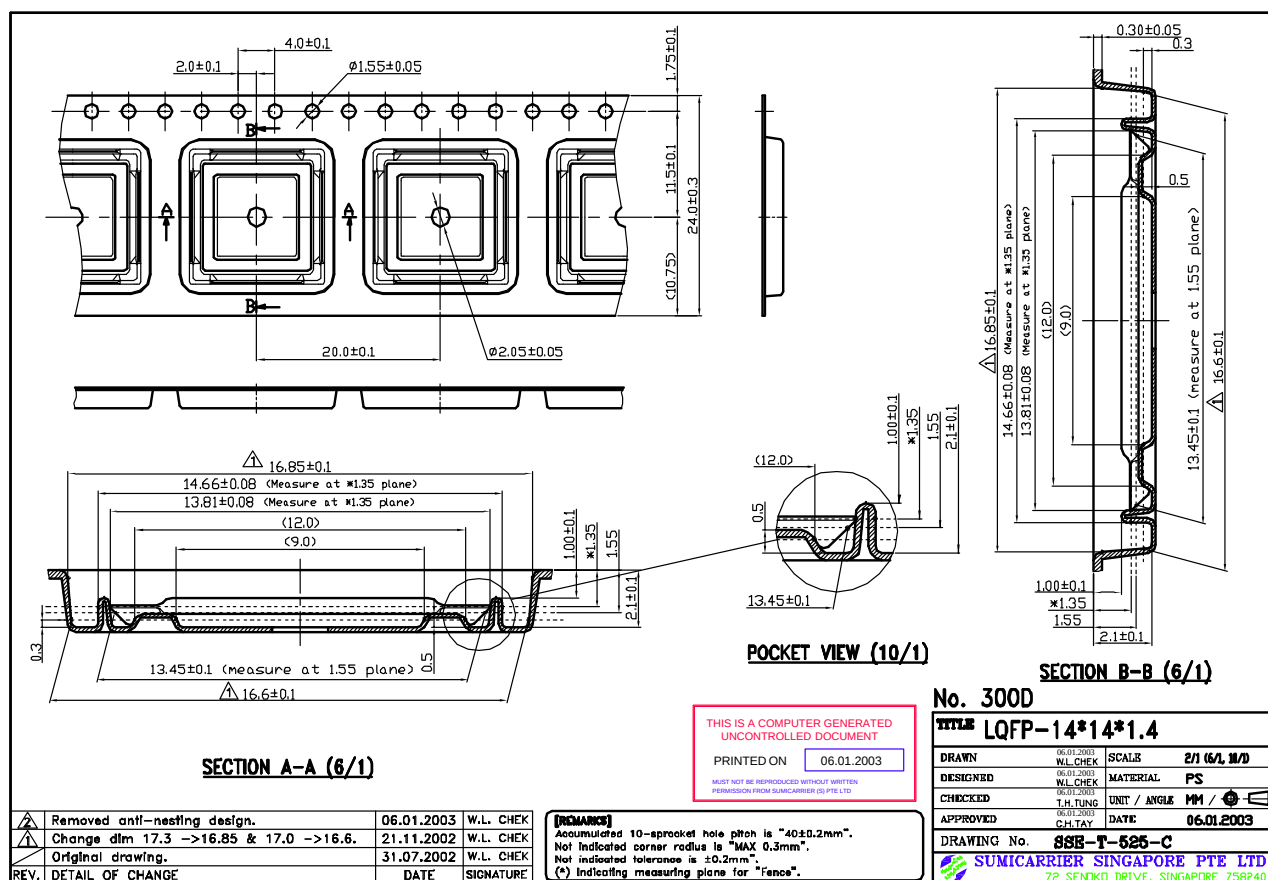
Figure D-6. 100-Pin LQFP Tape and Reel Dimensions
