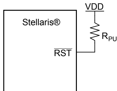
Figure 5-1. Basic RST Configuration
