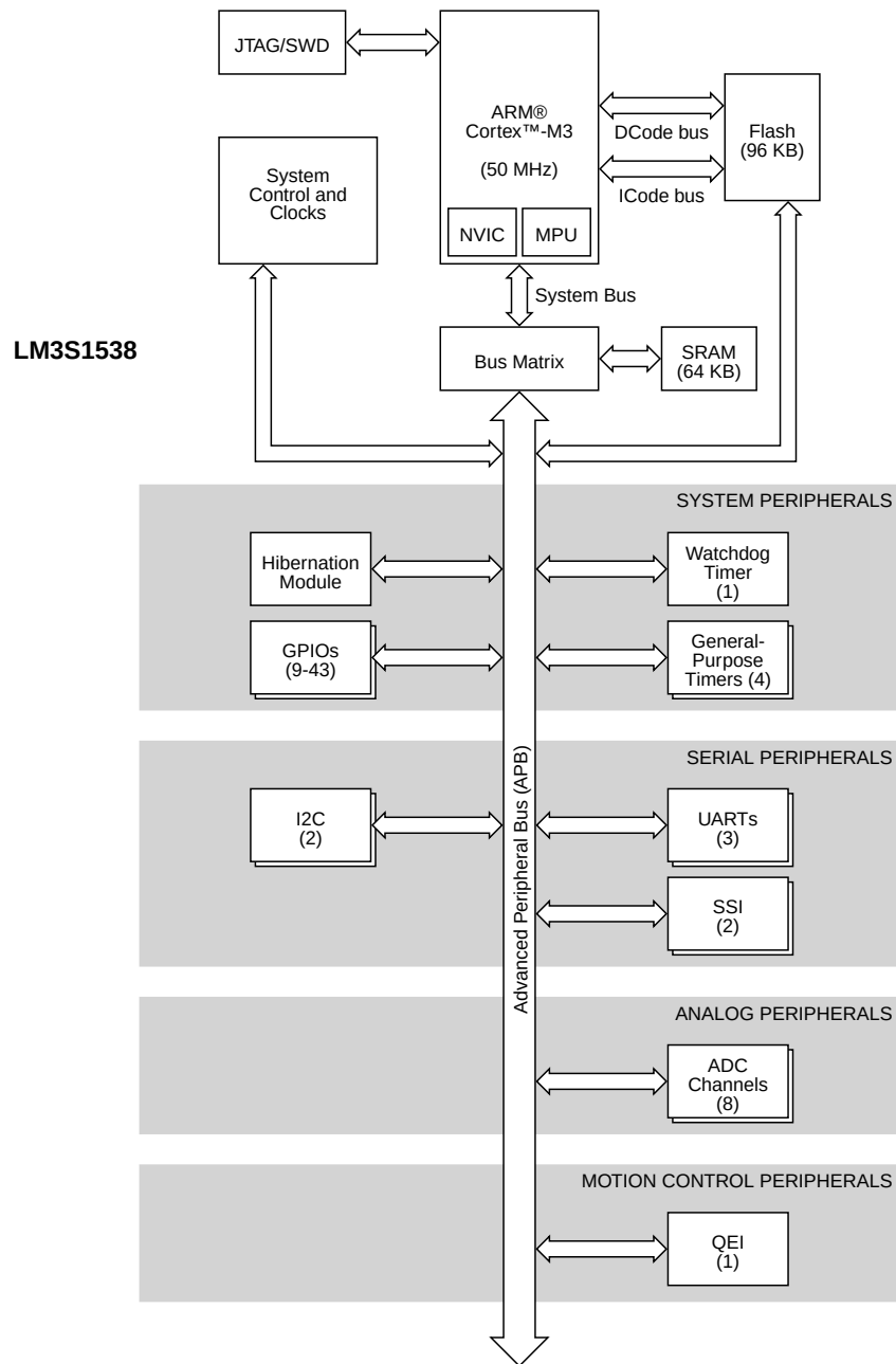
Figure 1-1. Stellaris® LM3S1538 Microcontroller High-Level Block Diagram
