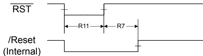
Figure 18-5. External Reset Timing ( \overline{RST} )
