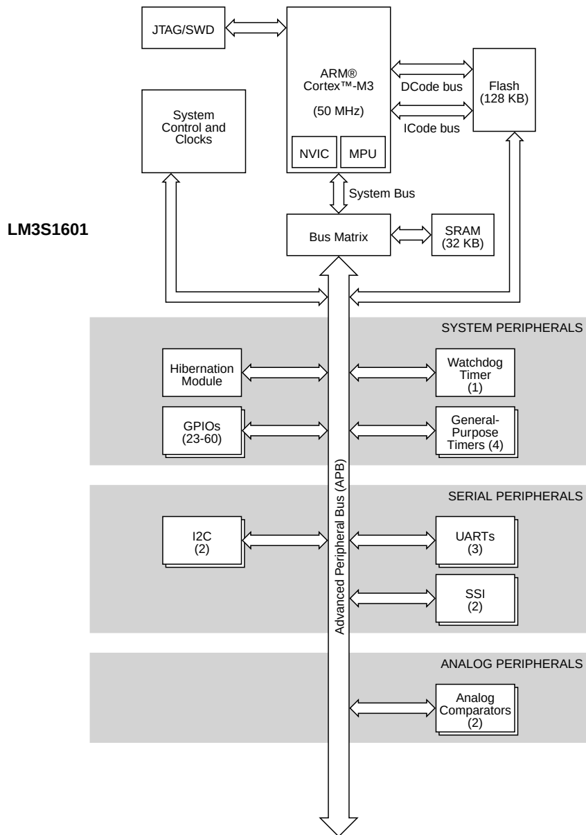
Figure 1-1. Stellaris® LM3S1601 Microcontroller High-Level Block Diagram
