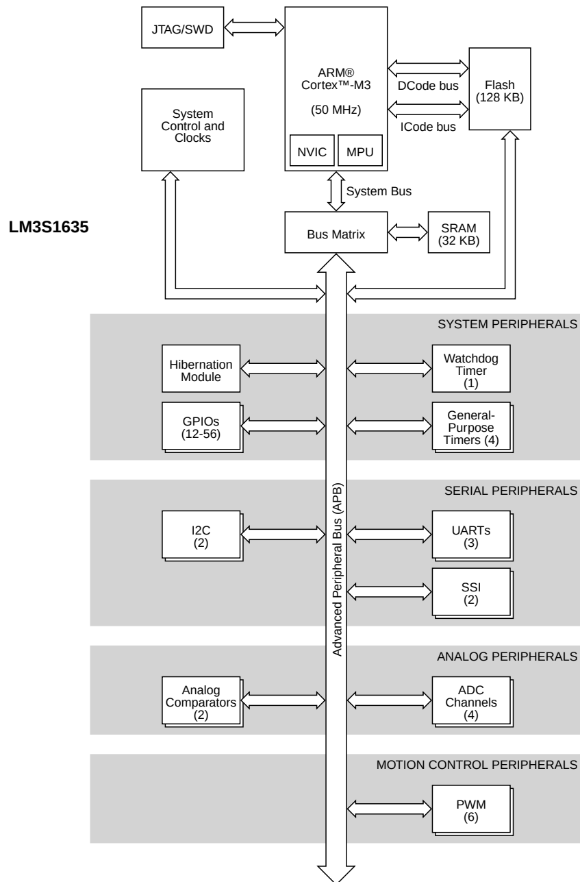
Figure 1-1. Stellaris® LM3S1635 Microcontroller High-Level Block Diagram
