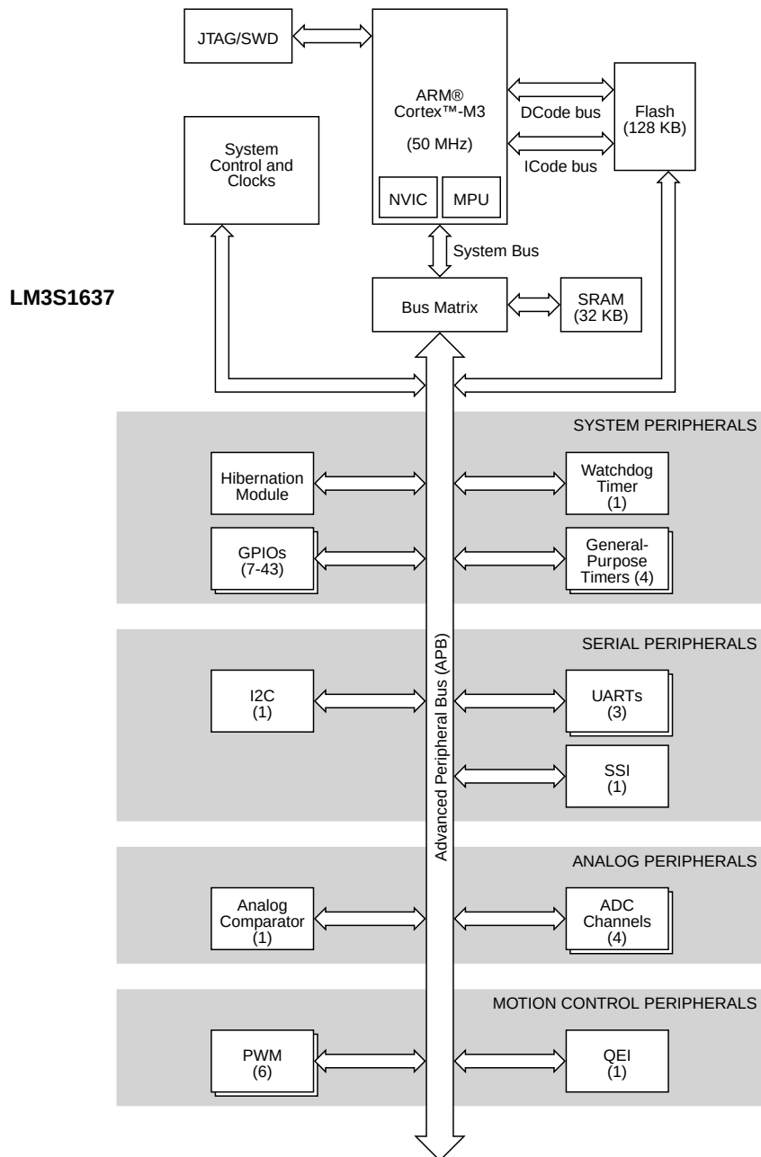
Figure 1-1. Stellaris® LM3S1637 Microcontroller High-Level Block Diagram
