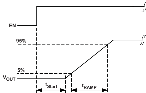
Figure 20. Soft Start
