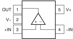
OPA376 SOT23-5 (TOP VIEW)
