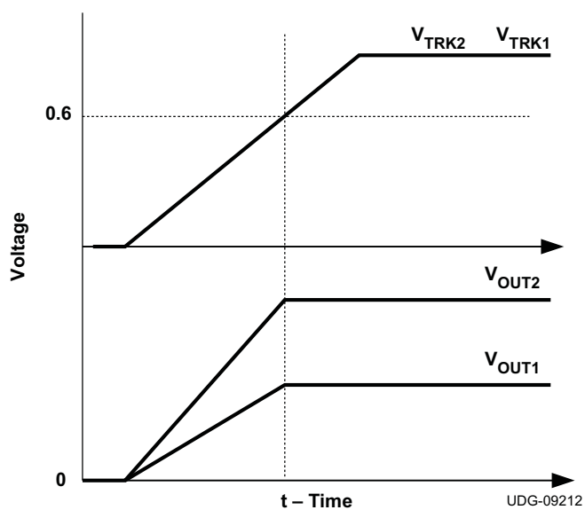
Figure 28. Ratiometric Voltage Tracking Waveform
