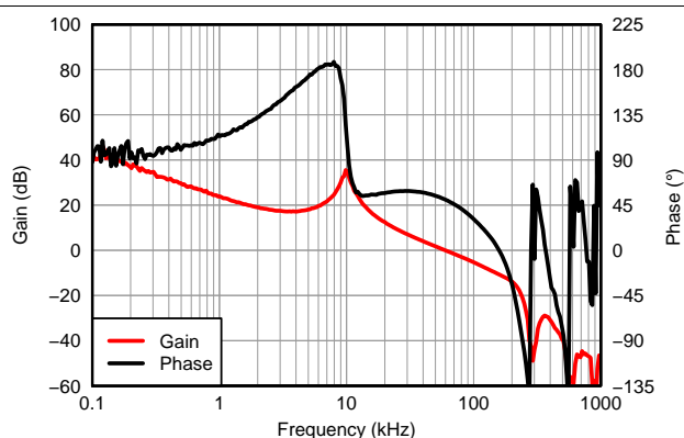
Figure 37. Loop Response
