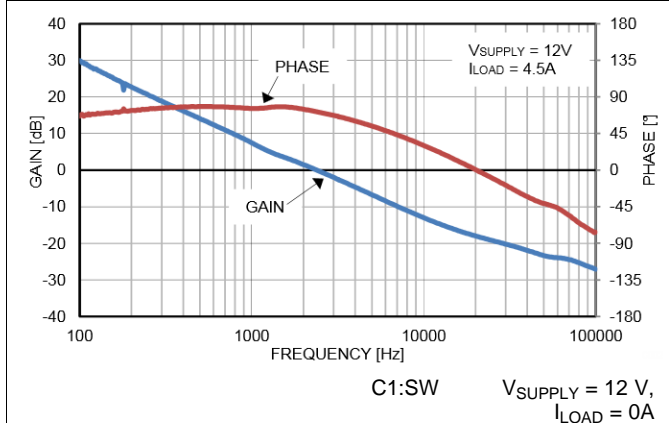
Figure 46. Loop Response
