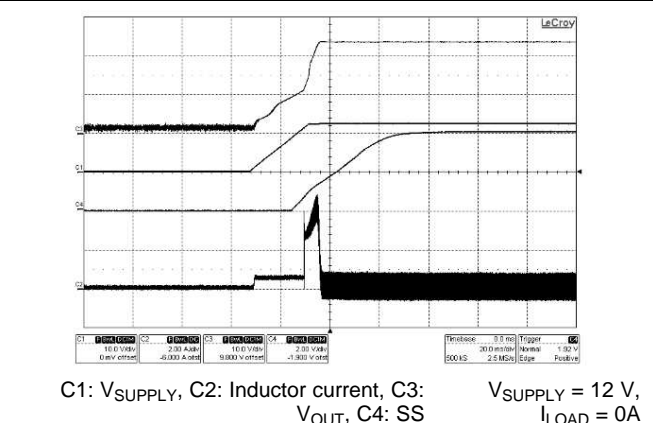
Figure 47. Start-Up
