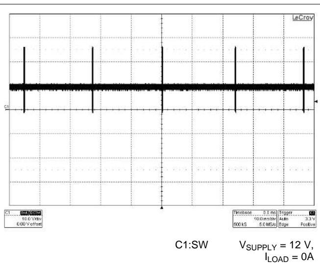
Figure 45. Skip Cycle
