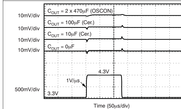
Figure 34. V_{BIAS} Line Transient (3 A)
