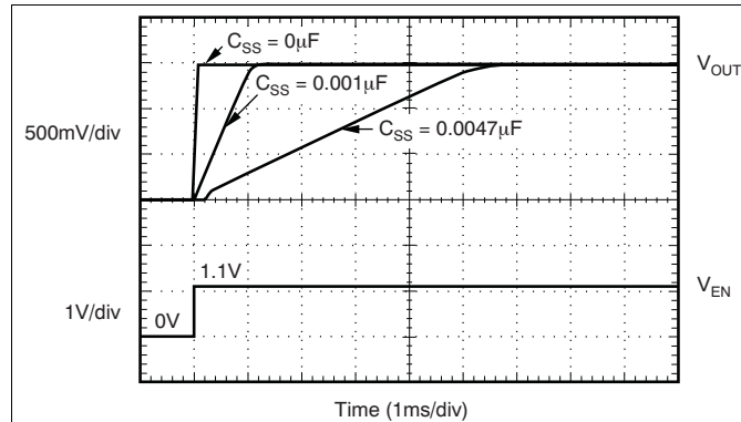
Figure 30. Turn-On Response
