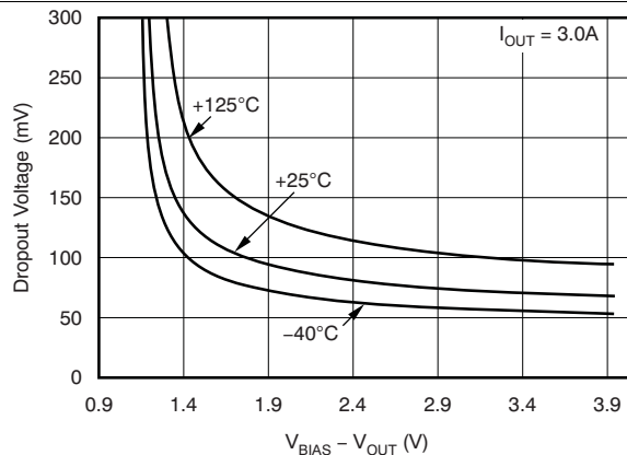
Figure 37. V_{IN} Dropout Voltage vs V_{BIAS} - V_{OUT} and Temperature ( T_J )
