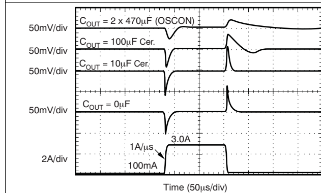
Figure 32. Load Transient Response
