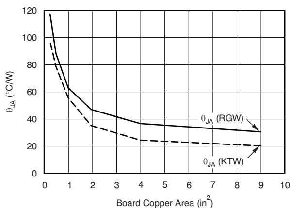
Figure 44. \theta_{JA} versus Board Size
