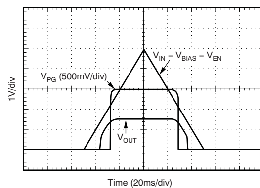
Figure 31. Power-Up, Power-Down
