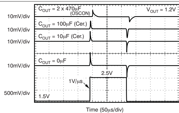
Figure 33. V_{IN} Line Transient (3 A)
