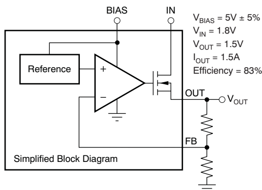
Figure 41. Typical Application of the TPS74401 Using an Auxiliary Bias Rail
