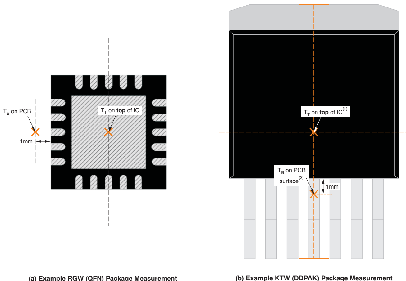
Figure 45. Measuring Points for T_T and T_B
