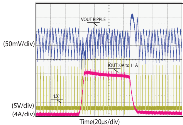
Transient Response - FCM (V_{DD} = 5\text{ V}, V_{IN} = 12\text{ V}, V_{OUT} = 1.5\text{ V}, I_{OUT} = 0\text{ A to } 11\text{ A}, \text{SiC401B}, dI/dt = 1\text{ A}/\mu\text{s})
