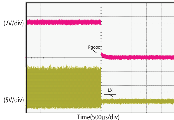
Over Temperature Shutdown at 133.4 °C (V_{IN} = 12\text{ V}, V_{OUT} = 1.5\text{ V}, I_{OUT} = 0\text{ A}, \text{LDO Mode}, \text{SiC401B})
